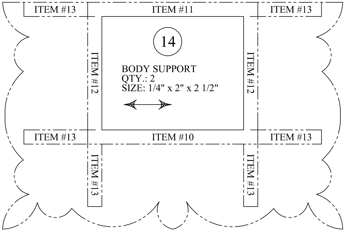
VIEW SHOWING BODY CROSS SECTION REF. SHEET 2 FOR ITEM #1 FLOOR
