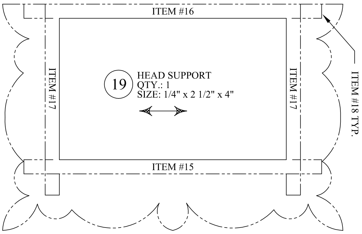
VIEW SHOWING HEAD CROSS SECTION REF. SHEET 2 FOR ITEM #1 FLOOR
